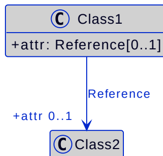
Figure 83. Graphical Representation of Shared Aggregation
