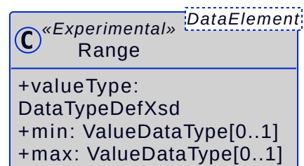
Figure 33. Metamodel of Ranges
