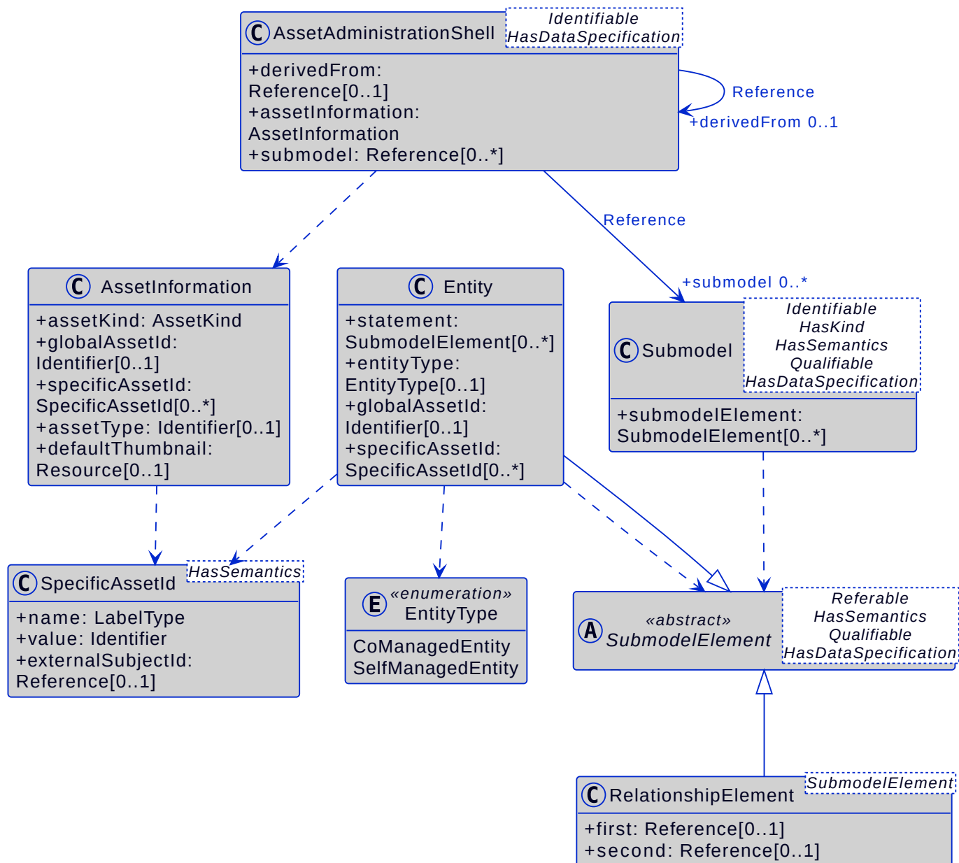
Figure 90. Extract From Metamodel for Composite I4.0 Components
