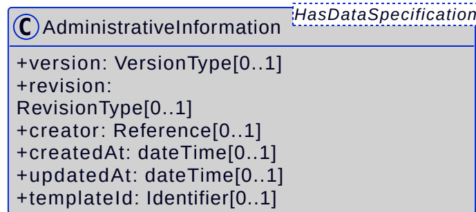
Figure 6. Metamodel of Administrative Information
