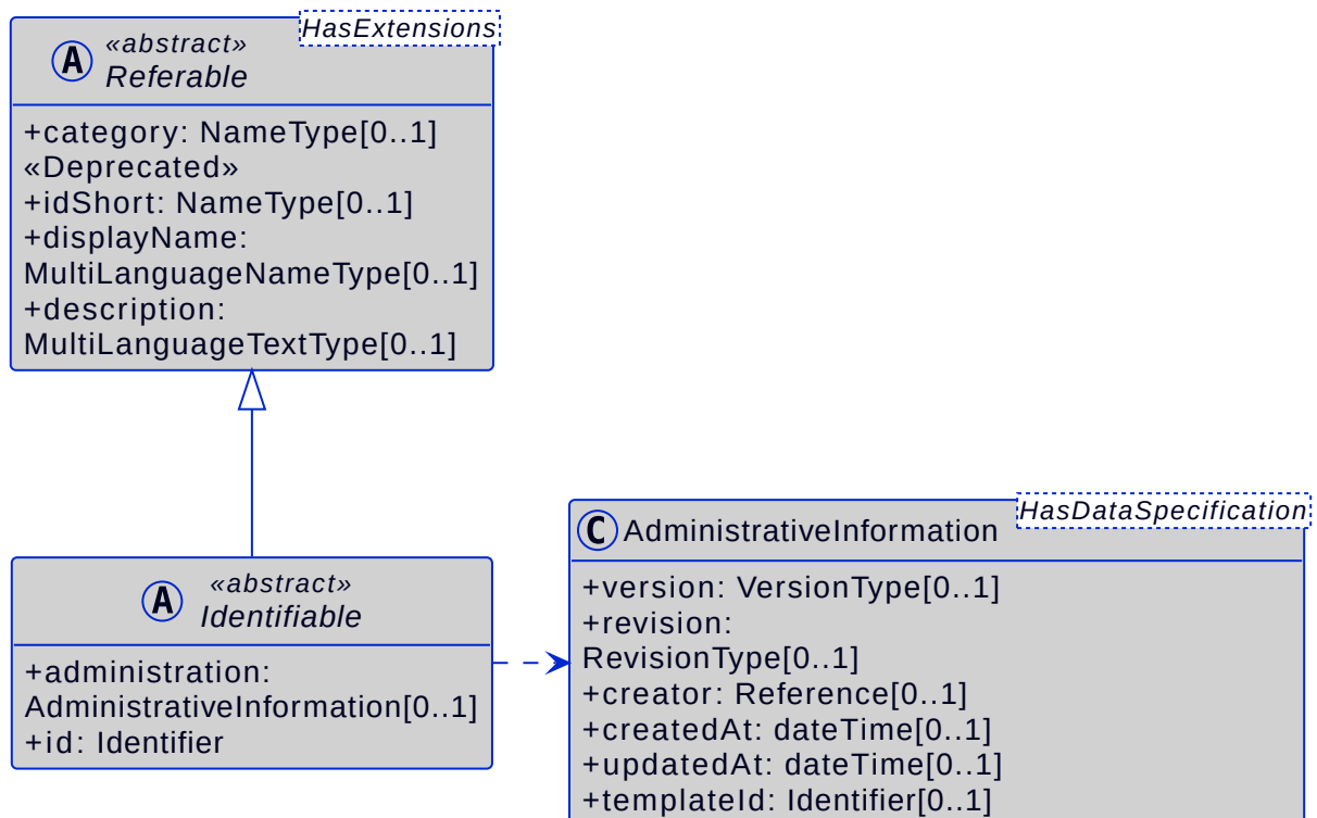
Figure 11. Metamodel of Identifiables
