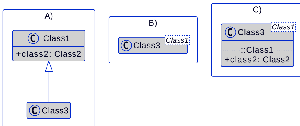
Figure 84. Graphical Representation of Generalization/Inheritance
