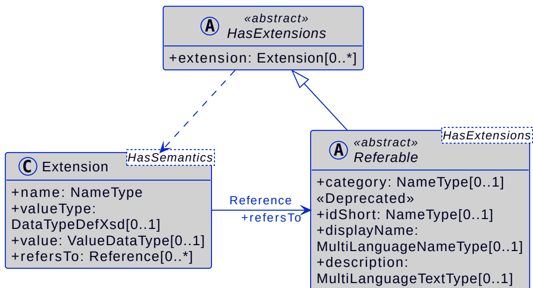
Figure 8. Metamodel of Has Extensions
