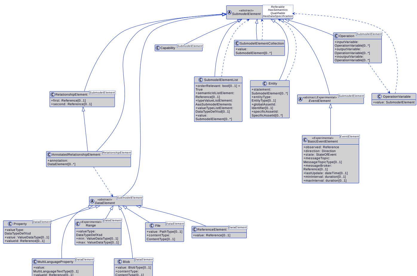
Figure 20. Metamodel Overview for SubmodelElement Subtypes
