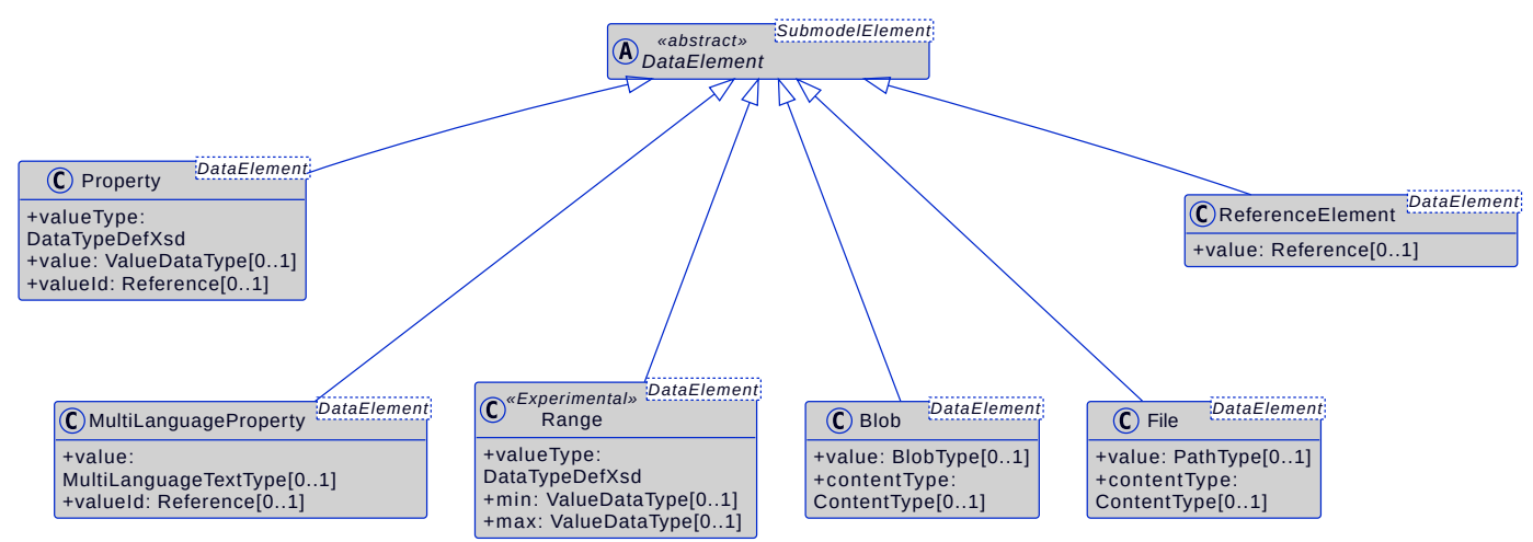
Figure 26. Metamodel of Data Elements
