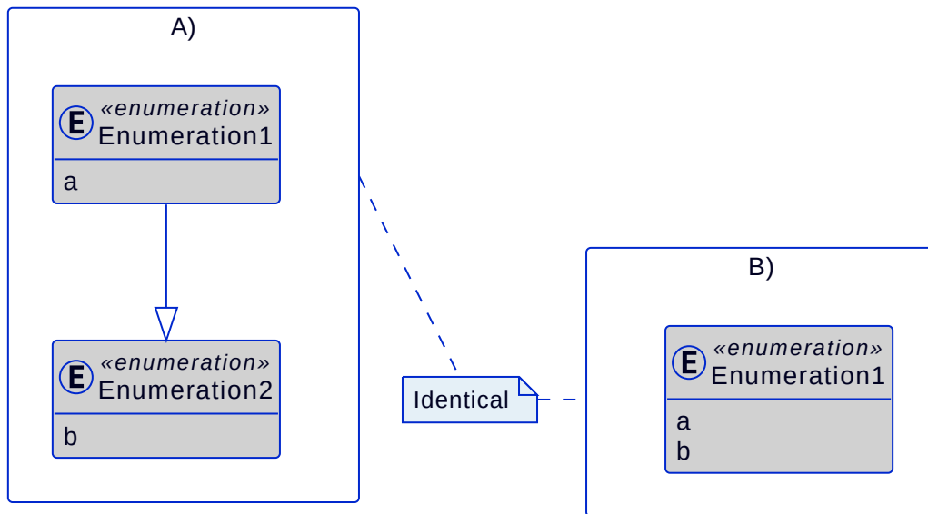
Figure 85. Graphical Representation for Enumeration with Inheritance
